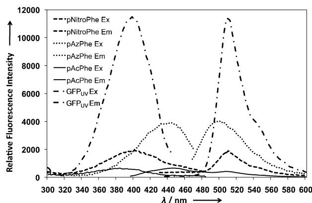
Figure 1. Fluorescence excitation (Ex) and emission (Em) spectra of GFP UV and UFPs containing different unnatural amino acids at position 66. The \lambda_{em}^{max} values are 508, 498, 442, and 510 nm for GFP UV , UFP-Tyr66pAzPhe, UFP-Tyr66pAcPhe, and UFP-Tyr66pNitroPhe, respectively. The \lambda_{ex}^{max} values are 395, 442, 384, and 400 nm for GFP UV , UFP-Tyr66pAzPhe, UFP-Tyr66pAcPhe, and UFP-Tyr66pNitroPhe, respectively. Fluorescence spectra were measured in phosphate buffer (50 mM, pH 7.4), and emission spectra were recorded with excitation wavelengths of each fluorescence protein's \lambda_{ex}^{max} .
